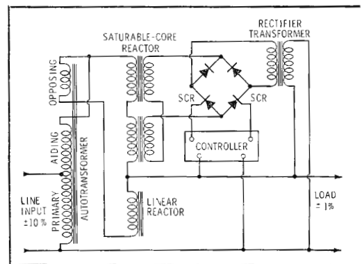
Fig. 2. Schematic diagram of voltage regulator employing saturable-core reactor.
