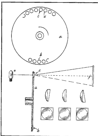
Fig. 1. Scanning lens disc system in which rotating lenses swept image across screen in horizontal direction, while the line was displaced vertically by changing angle of several successive prism elements.
