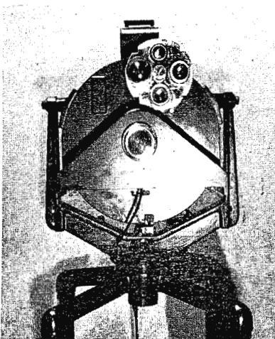
Fig. 2. 1931 flying spot scanner camera.
