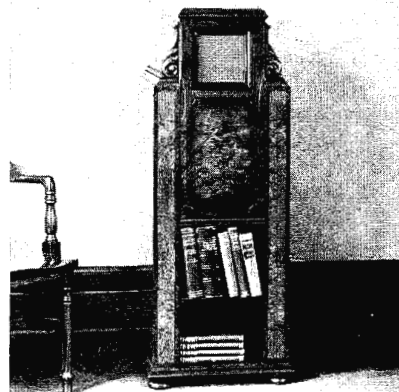
Fig. 10. Television receiver of 1931 to 34.
