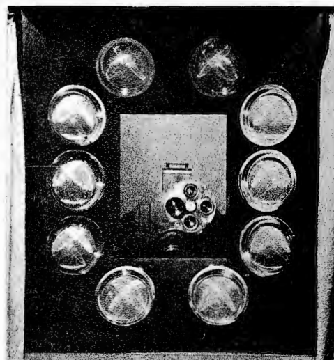
Fig. 4. Photocell bank used with flying spot scanner during 1931 to 34 at CKAC.
